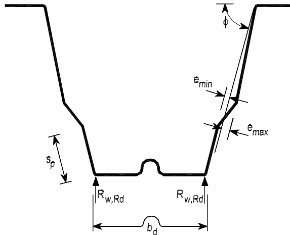
Figure 6.10: Stiffened webs
