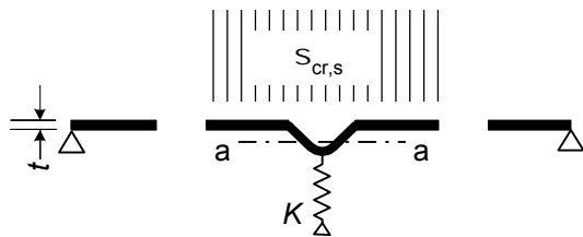
c) Step 2: Elastic critical stress S_{cr,s} for effective area of stiffener A_s from step 1
