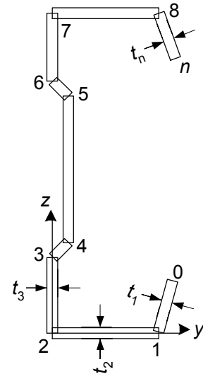
Figure C.1 Cross section nodes
