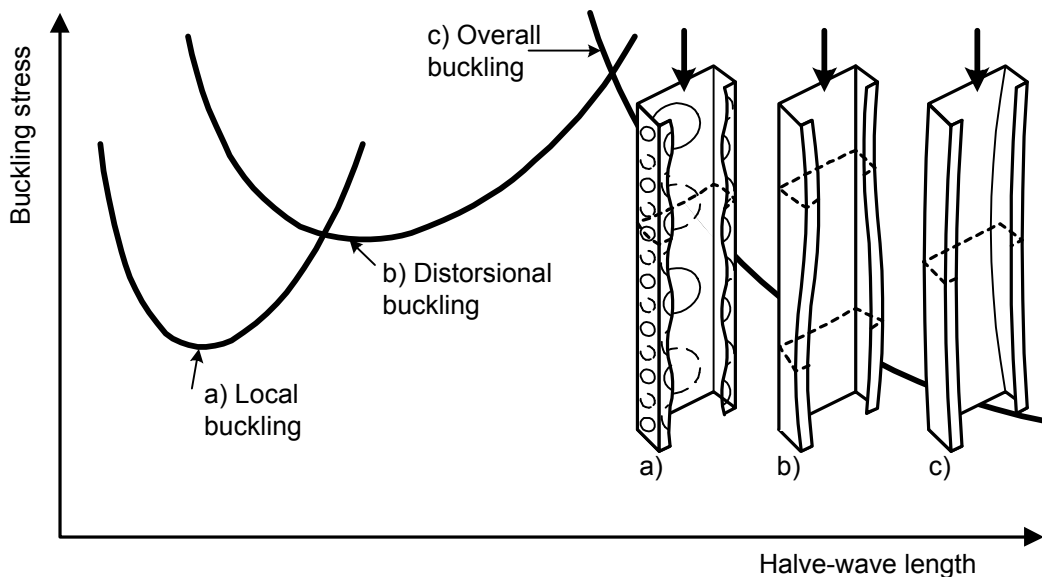
Figure 5.5a: Examples of elastic critical stress for various buckling modes as function of halve-wave length and examples of buckling modes.
