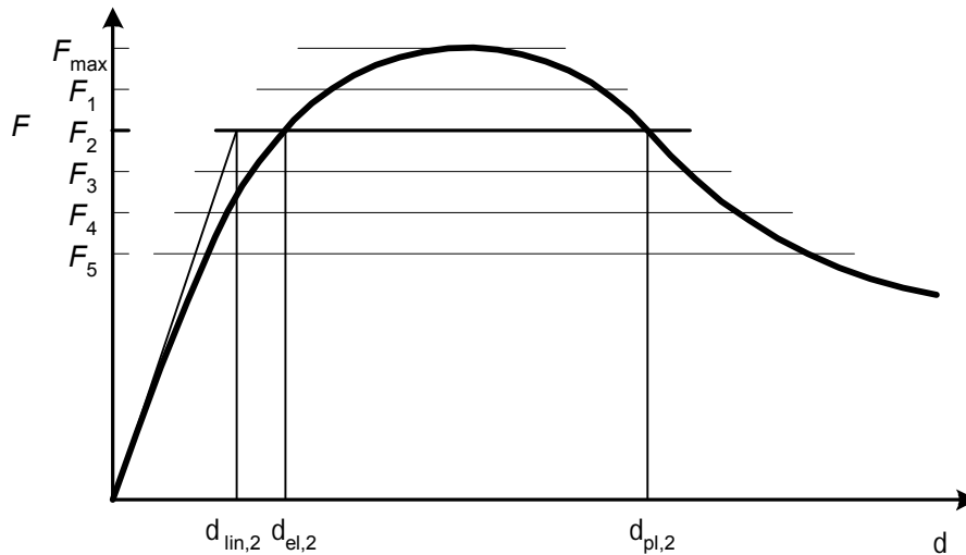
Figure A.9: Relation between load F and net deflection d
