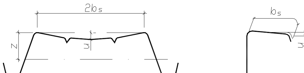
Figure 5.3: Flange curling
