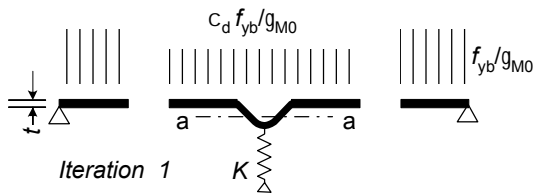
d) Reduced strength C_d f_{yb}/g_{M0} for effective area of stiffener A_s , with reduction factor C_d based on S_{cr,s}
