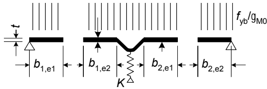
b) Step 1: Effective cross-section for K = \infty based on S_{com,Ed} = f_{yb}/g_{M0}
