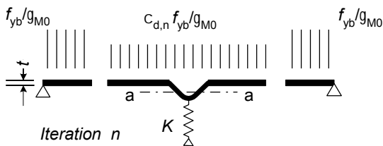
e) Step 3: Optionally repeat step 1 by calculating the effective width with a reduced compressive stress S_{com,Ed,i} = C_d f_{yb}/g_{M0} with C_d from previous iteration, continuing until C_{d,n} \approx C_{d,(n-1)} but C_{d,n} \leq C_{d,(n-1)} .
