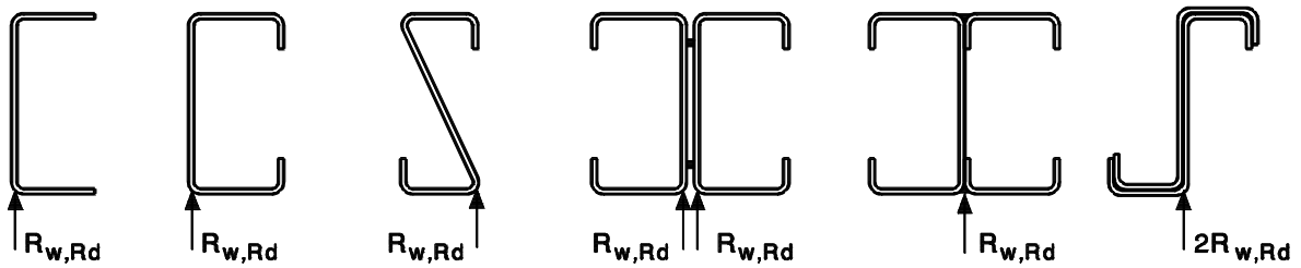
Figure 6.6: Examples of cross-sections with a single web
