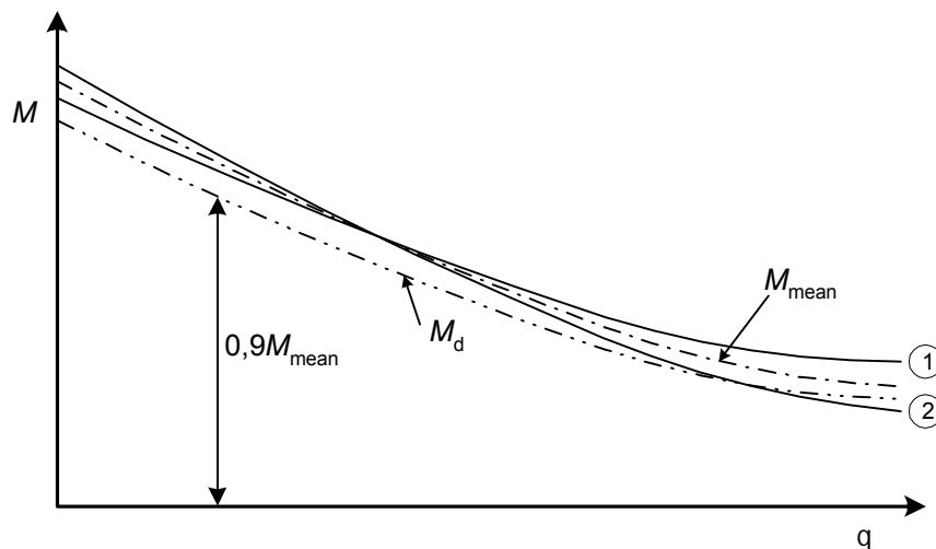
Figure A.10: Derivation of moment-rotation ( M - q ) characteristic
